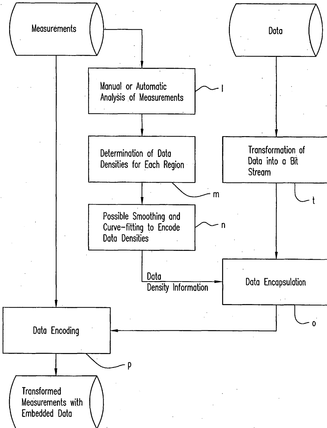
Variable Rate Data Encoding
